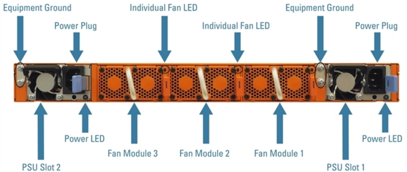
Figure 6 The GigaVUE TA Series-TA100-CXP Chassis Rear View
