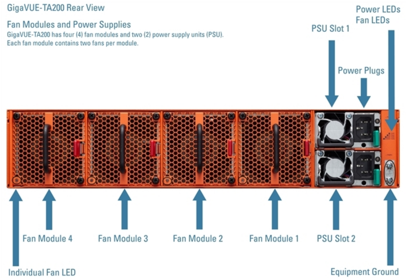
Figure 8 The GigaVUE TA Series-TA200 Chassis Rear View
