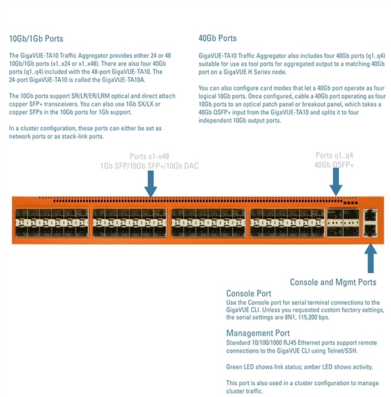
Figure 1 The GigaVUE TA Series-TA10 Chassis
